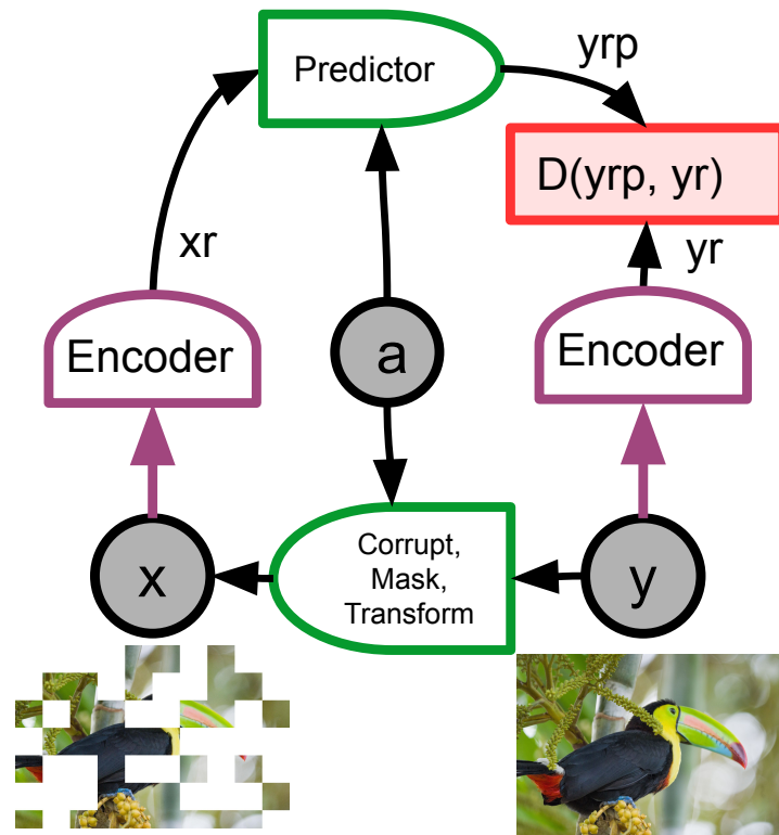
Joint Embedding Predictive Architecture (JEPA)
