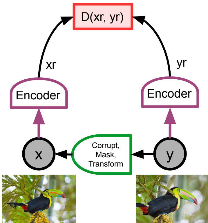
Joint Embedding Architecture, Siamese Networks
